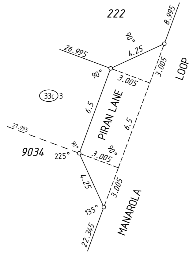
ENLARGEMENT 'B1' NOT TO SCALE
