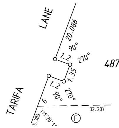
ENLARGEMENT 'B2' NOT TO SCALE
